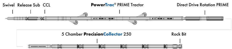
PRIME Enhanced PrecisionCollector Toolstring
