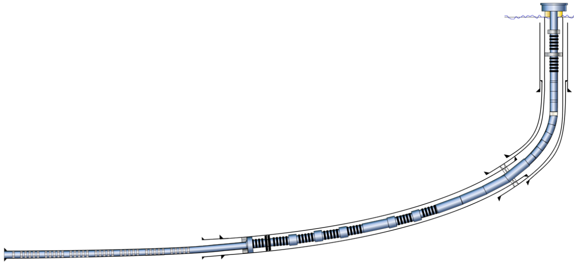
Multi-stage Frac Sleeve Completion
