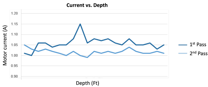
Motor current observed during job execution
