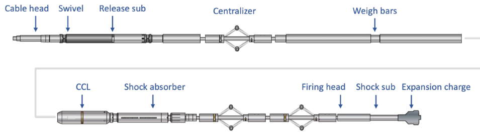
Expansion charge toolstring
