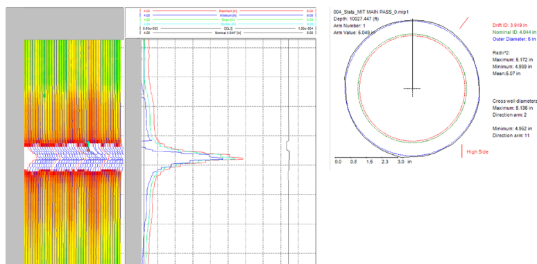
Multi-finger Caliper log data showing the resulting ID of the 5 in. tubing after expansion
