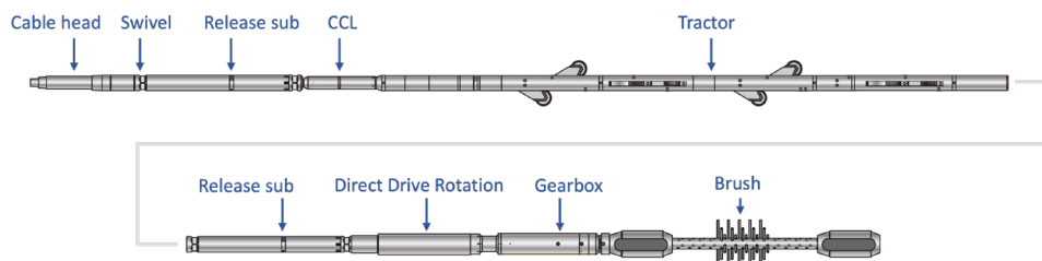
Tubing cleaning toolstring
